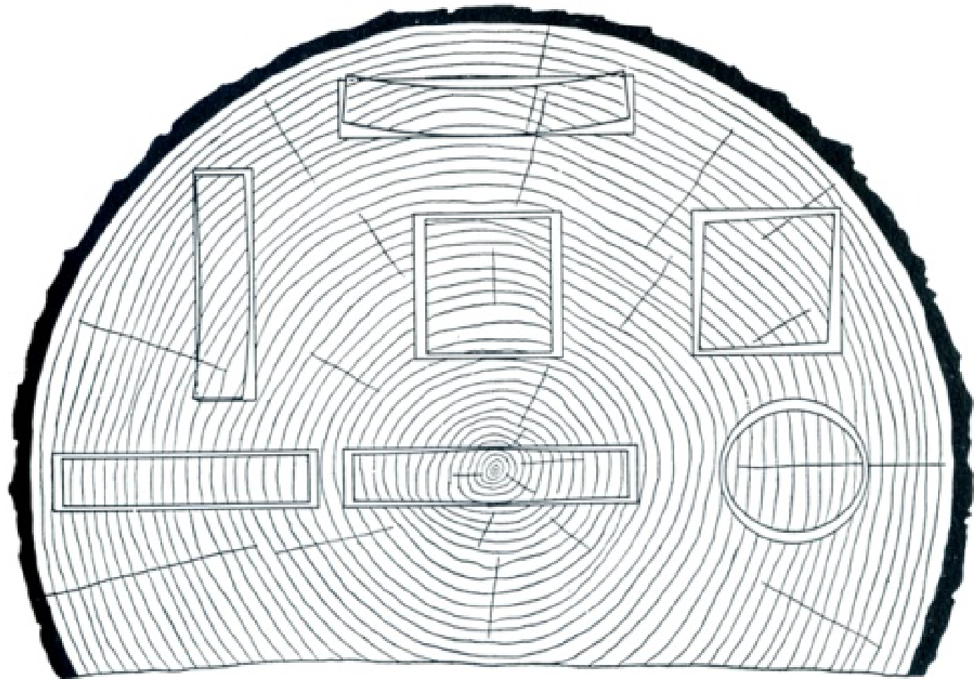
Characteristic shrinkage and distortion of flats, squares, and rounds as affected by the direction of the annual rings
